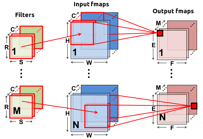
Fig. 1. Computation of a CNN layer.
